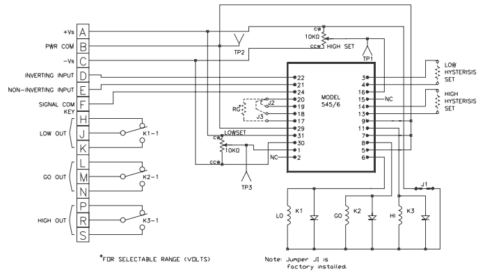
FIGURE 17. MK379 Circuit Drawing
