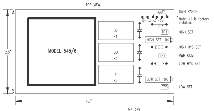
FIGURE 18. MK379 Outline Drawing
