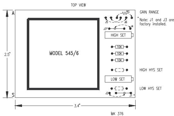
FIGURE 11. MK376 Outline Drawing
