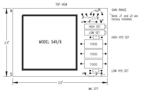
FIGURE 13. MK377 Outline Drawing
