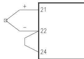
FIGURE 2. Single-Ended Connections
