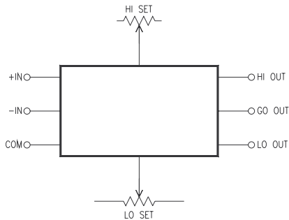
FIGURE 1. Simplified Diagram for Models 545 and 546
