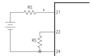
FIGURE 3. High Source Impedance Connections
