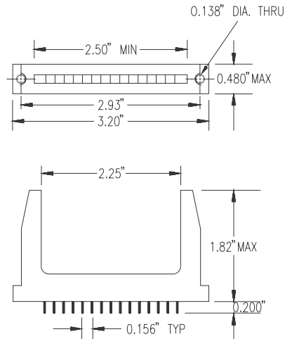
FIGURE 16. 15-pin Mating Connector for Model 545/546 Mounting Kits.
