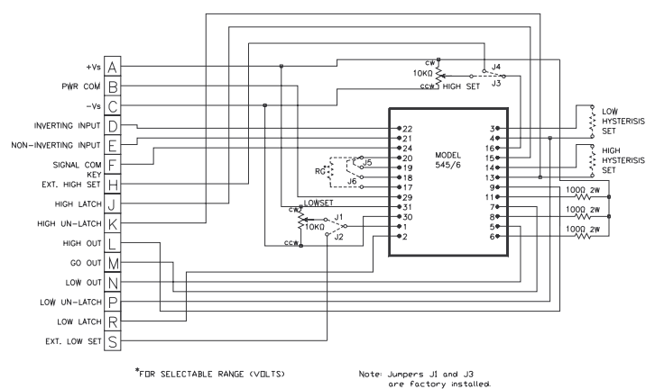
FIGURE 12. MK377 Circuit Drawing
