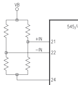
FIGURE 4. Bridge Differential Connection
