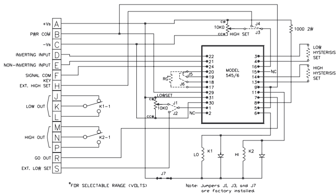
FIGURE 14. MK378 Circuit Drawing
