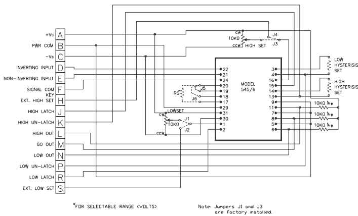
FIGURE 10. MK376 Circuit Drawing
