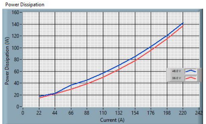
Fig. 2: 48S12.3K0BCA Power Dissipation – Buck Mode, V_o=14V .
