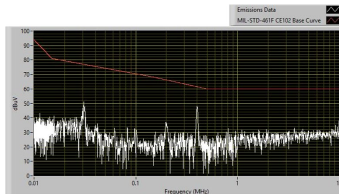
b) With input filter from Fig. 47.
