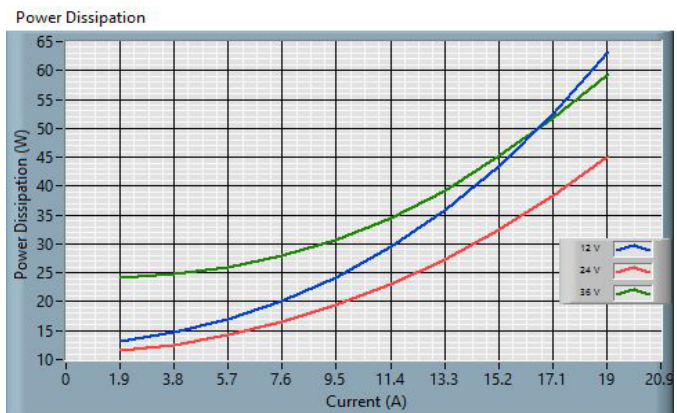
Fig. 16: 24S53.19FXW (ROHS) Power Dissipation
