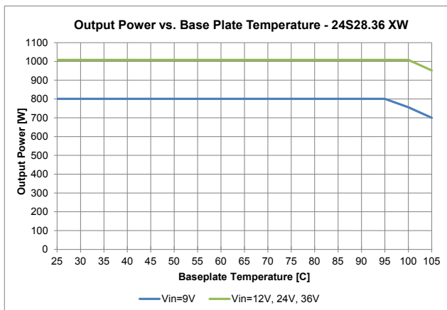
Fig. 21: 24S28.36FXW (ROHS) Derating Curve
