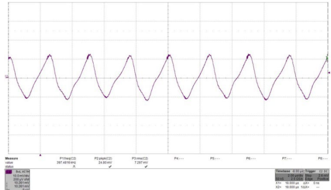
Fig. 32: Input reflected ripple current, i_c (500mA/mV), measured at input terminals at full rated load current at V_{in} = 24V . Refer to Fig. 2 for test setup. Time: 2 \mu s /div. RMS input ripple current is 7.3 \times 0.5A = 3.65A_{RMS} .
