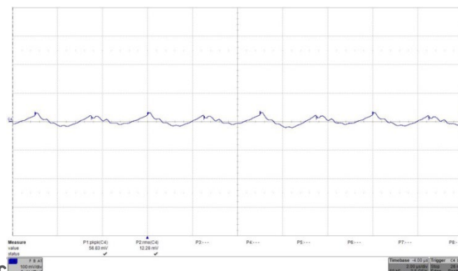
Fig. 49: Output voltage ripple (100 mV/div.) at full rated load current into a resistive load at V_{in} = 24V . Time: 2 \mu s /div.
